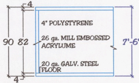
SECTION VIEW
